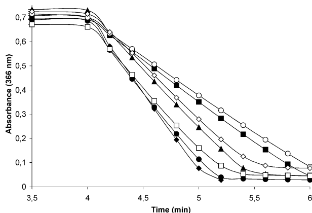
Figure 3. GSH Px-like activity of diselenides. Reactions were initiated by addition of 1.0 mM \text{H}_2\text{O}_2 to the assay mixture containing 1.0 mM GSH, 0.26 mM NADPH, 1 U/mL GSSG reductase and 50 \mu\text{M} compound 4f ( \blacklozenge ), compound 4h ( \bullet ), compound 4j ( \blacktriangle ), compound 4i ( \blacksquare ), compound 4k ( \circ ), compound 4b ( \square ) and compound 4e ( \diamond ).
