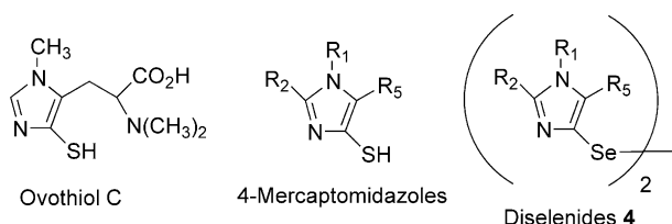
Figure 1. Structures of ovothiol C, 4-mercaptoimidazoles and imidazole diselenides.
