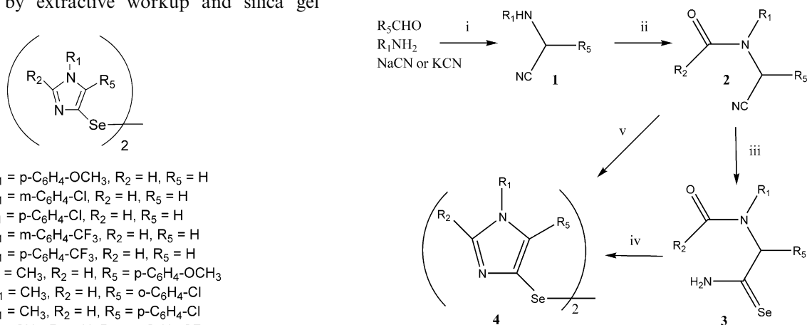
Scheme 1. Reagents and conditions: (i) \text{H}_2\text{O} – \text{MeOH} , \text{HCl} or \text{AcOH} ; (ii) \text{HCO}_2\text{H} – \text{Ac}_2\text{O} or \text{RCOCl} , \text{Et}_3\text{N} ; (iii) \text{Al}_2\text{Se}_3 , \text{H}_2\text{O} , \text{Et}_3\text{N} ; (iv) \text{Me}_3\text{SiOTf} , \text{CH}_2\text{Cl}_2 , \text{Et}_3\text{N} , -10^{\circ}\text{C} ; (v) \text{Se} , \text{NaBH}_4 , \text{EtOH} , \text{Et}_3\text{N} , room temperature then slight reflux.
