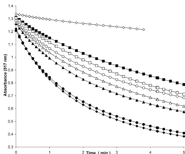
Figure 4. DPPH scavenging (initial concentration 100 \mu\text{M} ) by an ethanolic solution of 100 \mu\text{M} glutathione and 50 \mu\text{M} compound 4f ( \blacklozenge ), compound 4h ( \bullet ), compound 4j ( \blacktriangle ), compound 4i ( \blacksquare ), compound 4a ( \triangle ), compound 4d ( \square ), compound 4k ( \circ ) and diphenyldiselenide ( \diamond ).
